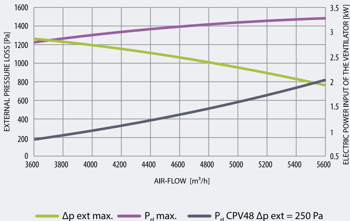
Maximum external pressure CPV48 standard – inlet part
