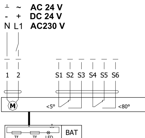
Obr. 15 Servopohon BELIMO BF 230-TN, BF 24-TN (-ST)
