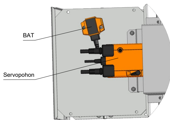
Obr. 13 Servopohon BELIMO BFL (BFN) 230-T
