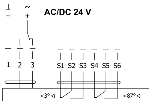
Obr. 11 Servopohon BELIMO BE 24-12(-ST)
