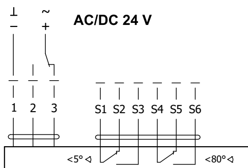
Obr. 9 Servopohon BELIMO BEE 24(-ST)
