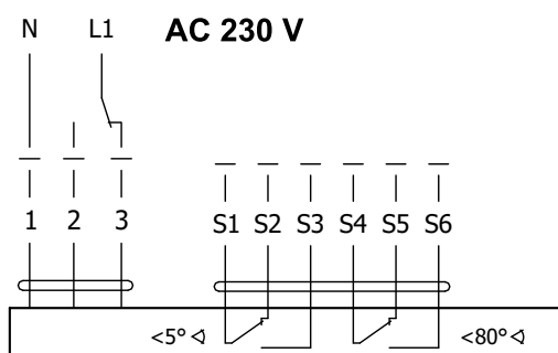
Obr. 8 Servopohon BELIMO BEN 230
