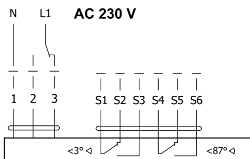
Obr. 12 Servopohon BELIMO BE 230-12
