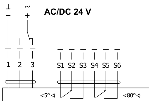
Obr. 7 Servopohon BELIMO BEN 24(-ST)
