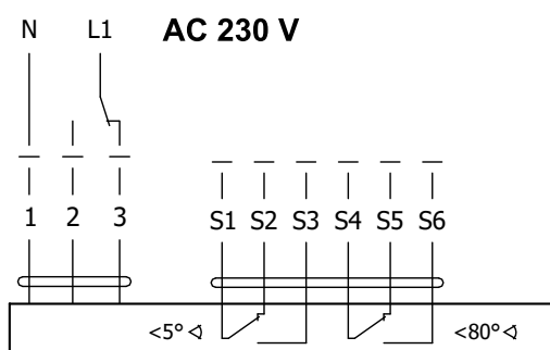
Obr. 10 Servopohon BELIMO BEE 230
