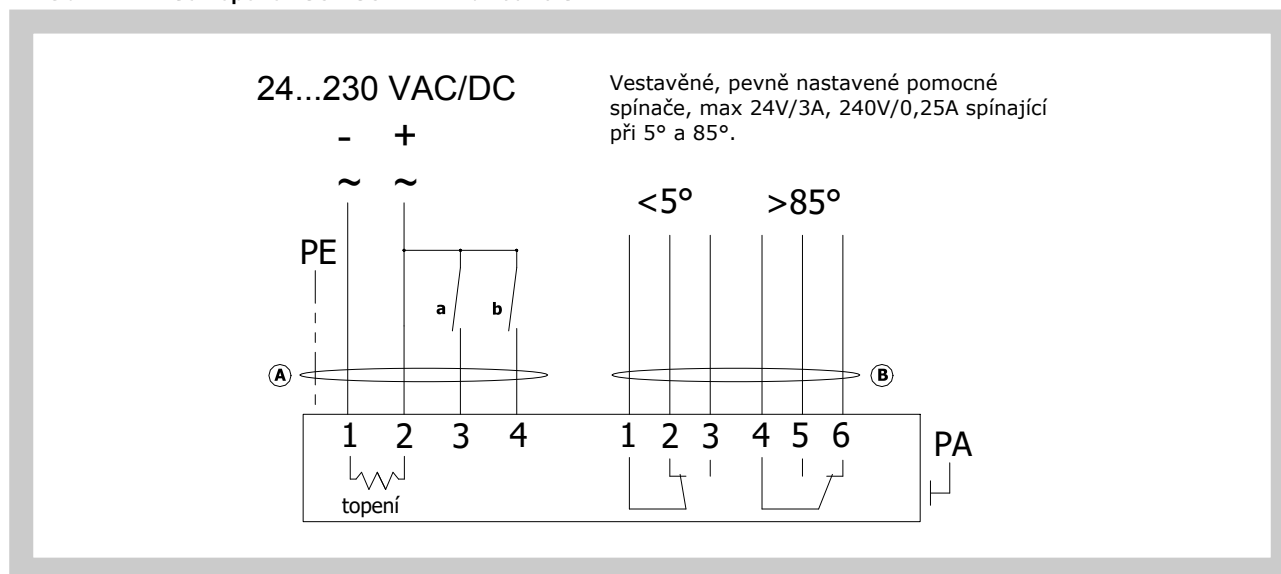
Obr. 12 Servopohon SCHISCHEK InMax 50.75-S
