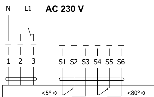
Obr. 9 Servopohon BELIMO BEE 230
