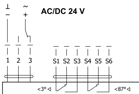
Obr. 10 Servopohon BELIMO BE 24-12(-ST)
