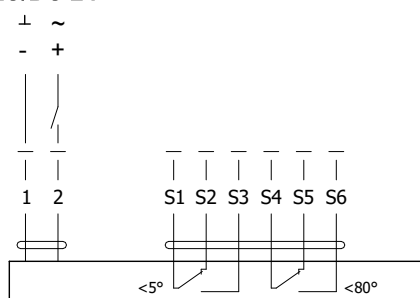
Obr. 15 Servopohon BELIMO BFN 230
