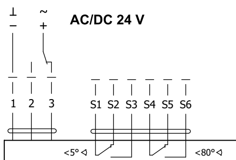
Obr. 7 Servopohon BELIMO BEE 24(-ST)
