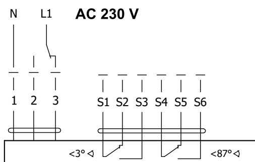
Obr. 11 Servopohon BELIMO BE 230-12
