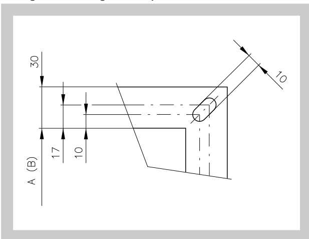
Fig. 24 Flange of Damper
