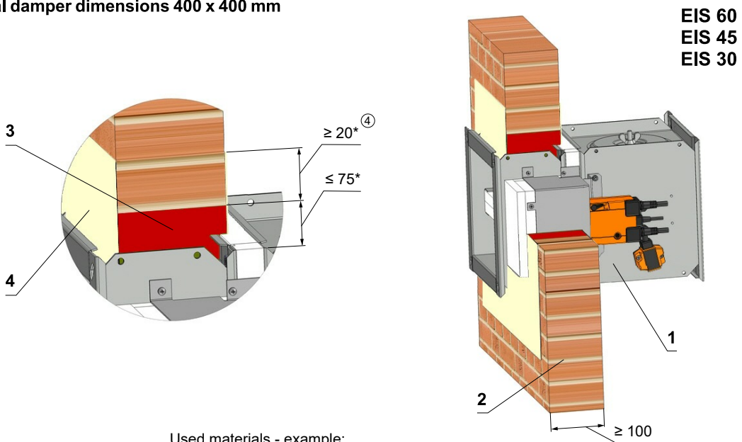
Fig. 29 Solid wall construction - fire protection foam with stucco plaster
