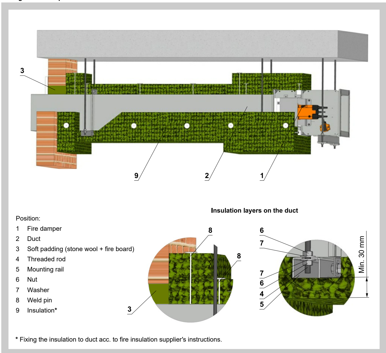
Fig. 52 Suspension remote from the wall - horizontal installation
