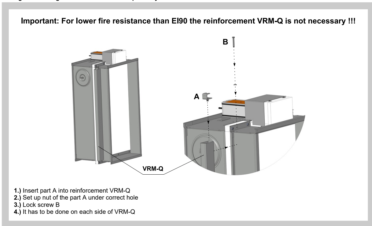
Fig. 47 Fixing of reinforcement to damper body
