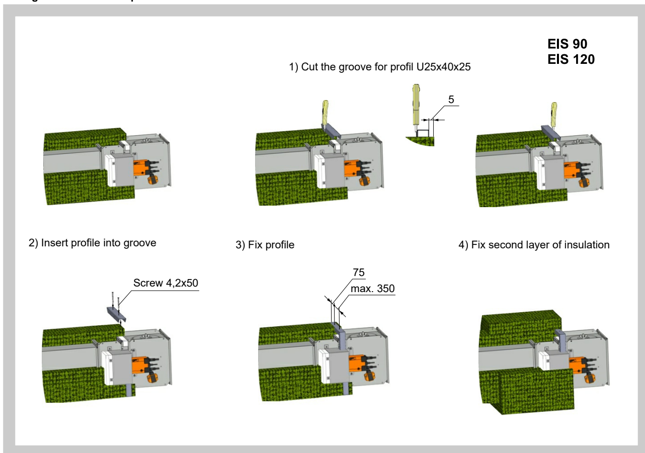
Fig. 48 Installation procedure
