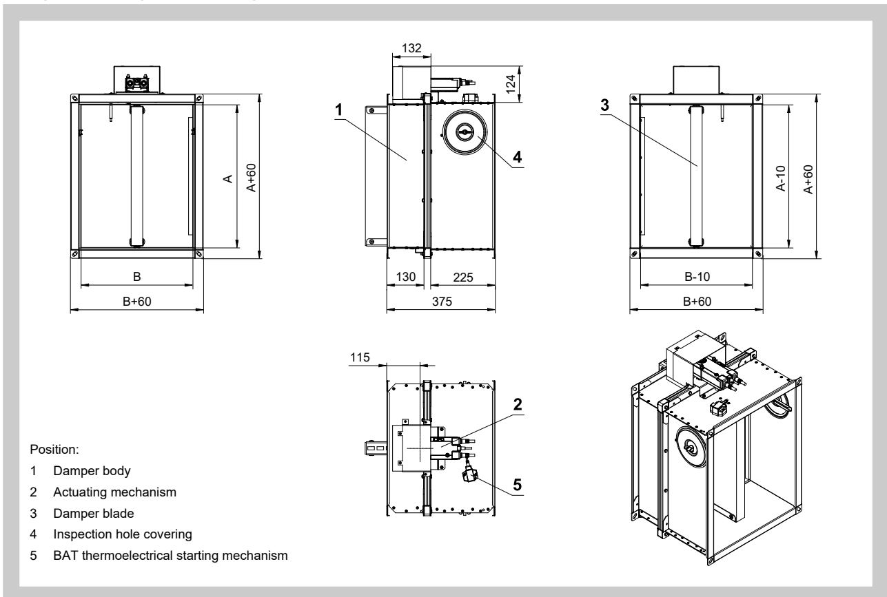
Fig. 22 Design with actuating mechanism
