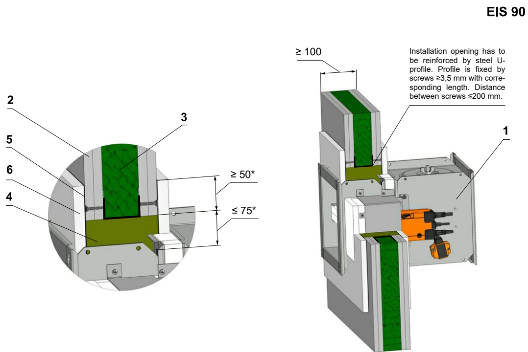
Fig. 38 Gypsum wall construction - stuffing box, fire protection mastic and cement lime plate
