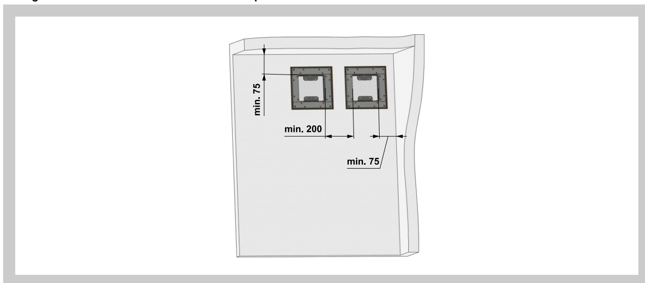
Fig. 25 The distance between the fire damper and the construction
