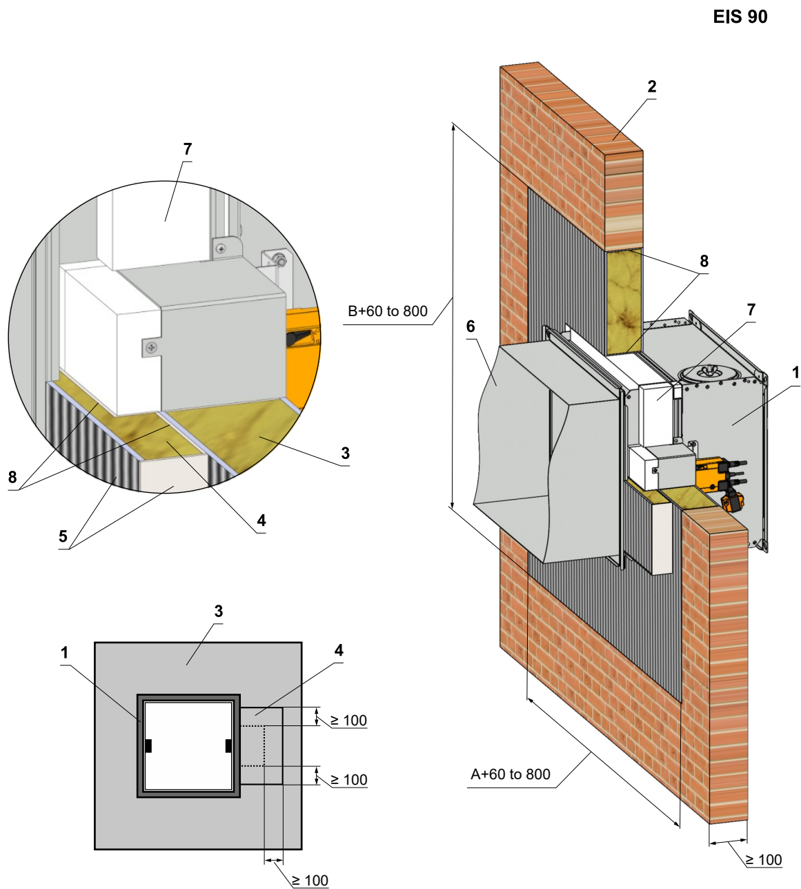
Fig. 32 Solid wall construction - Ablative Coated Batt
