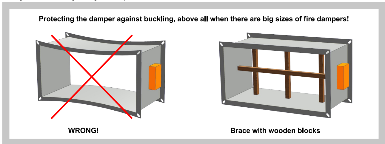
Fig. 53 Embedding / fixing the damper
