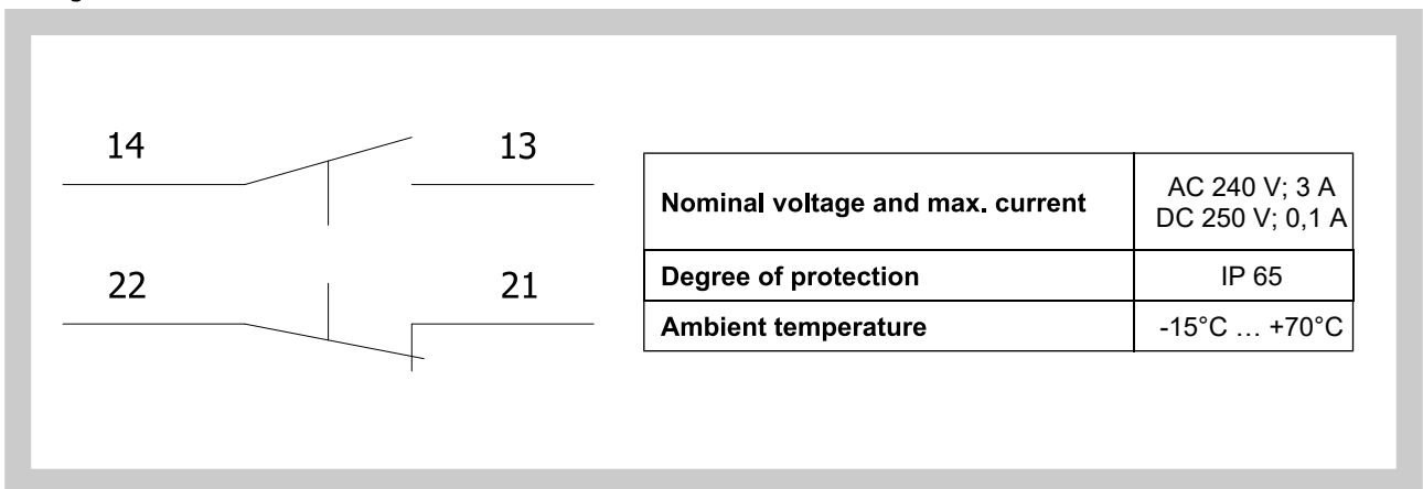
Fig. 5 Limit switch XCKN2118G-11
