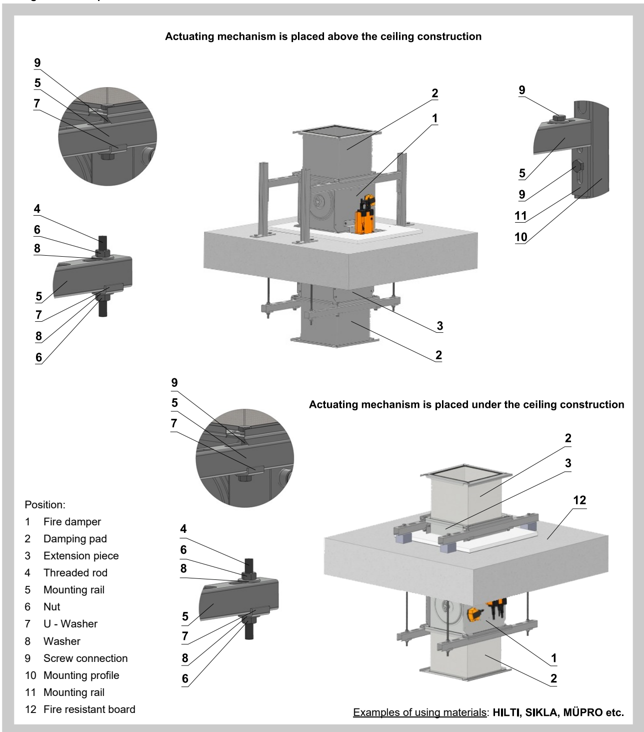
Fig. 51 Suspension - vertical duct
