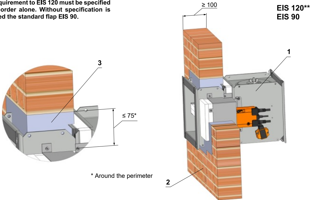
Fig. 28 Solid wall construction - mortar or gypsum
