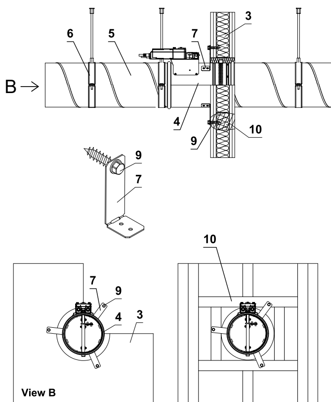
In gypsum wall construction
