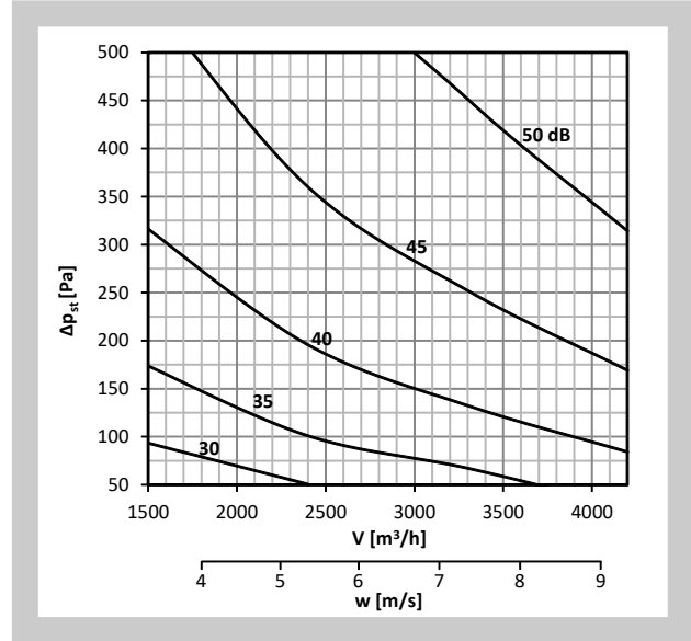
Diagram No. 62 Sound power level L_{WA} [dB(A)] radiated outside the pipeline 500x400, with insulation
