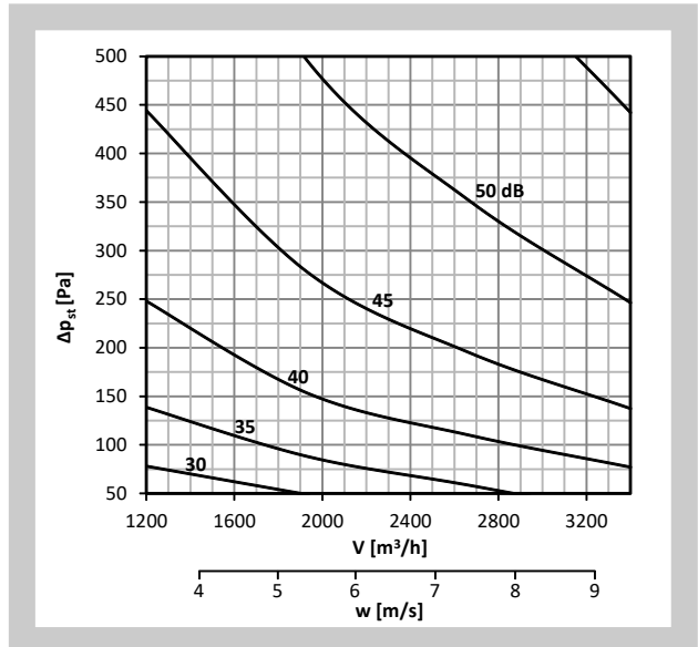
Diagram No. 58 Sound power level L_{WA} [dB(A)] radiated outside the pipeline 400x400, with insulation
