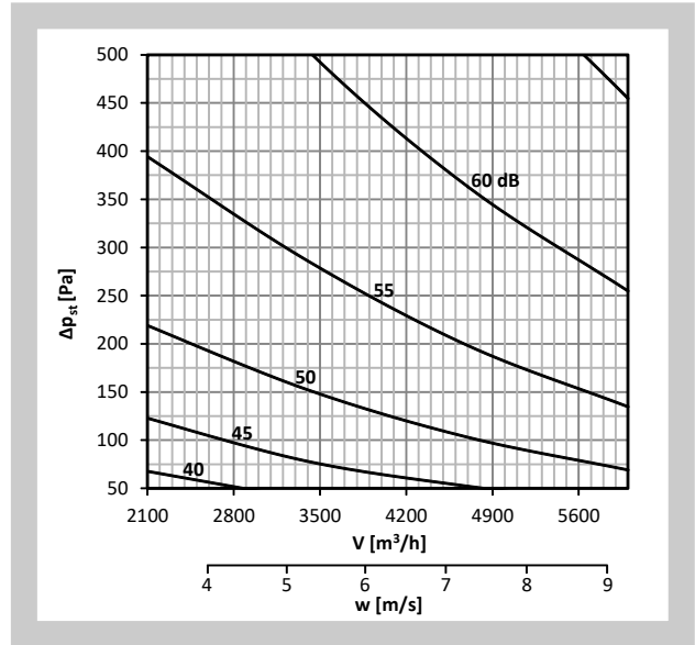
Diagram No. 45 Sound power level L_{WA} [dB(A)] radiated outside the pipeline 600x500, without insulation
